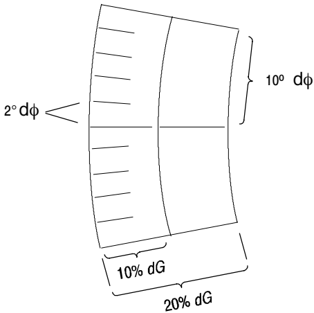
Figure 3-6: Differential gain and phase measurement box
