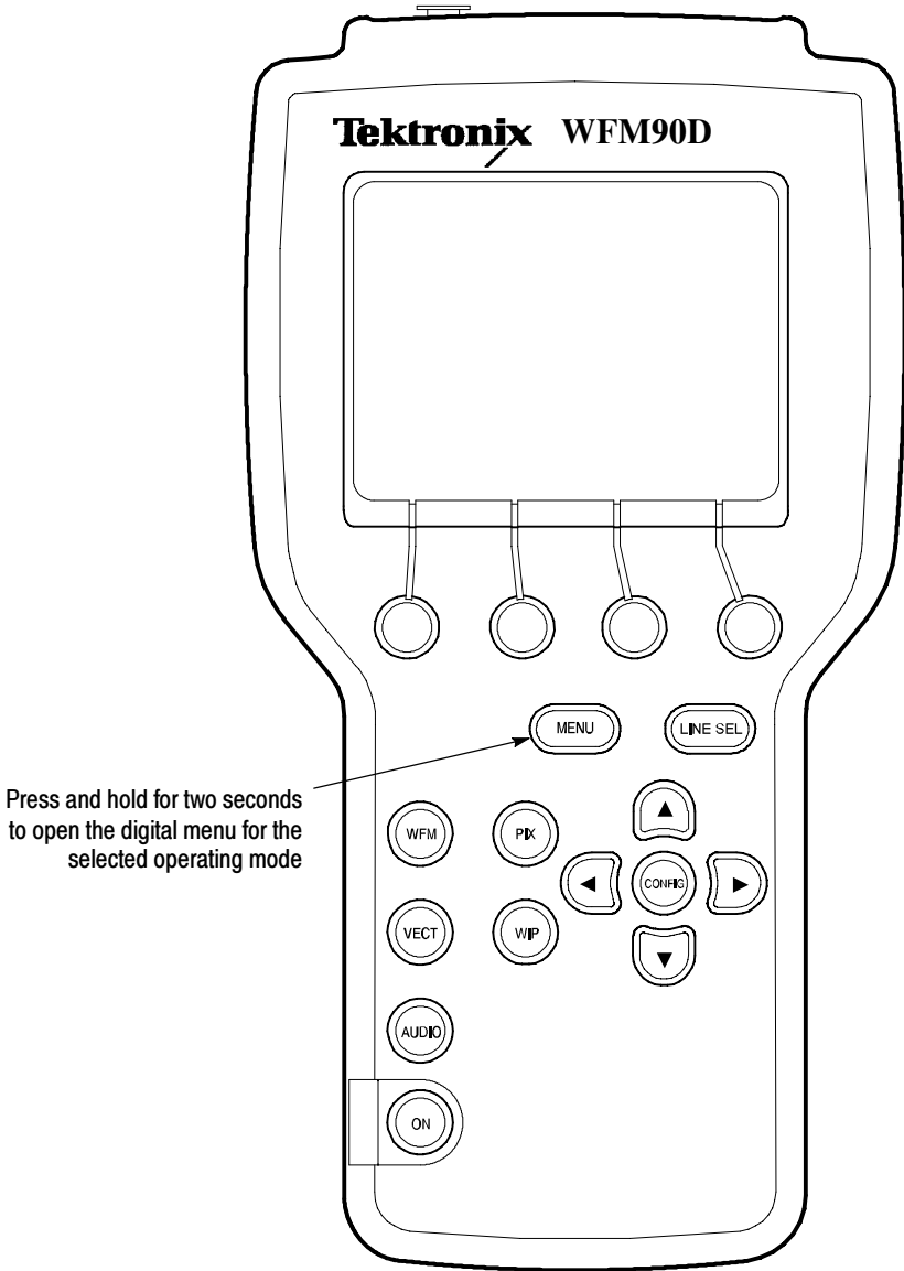
Figure 2- 1: WFM90D keypad
