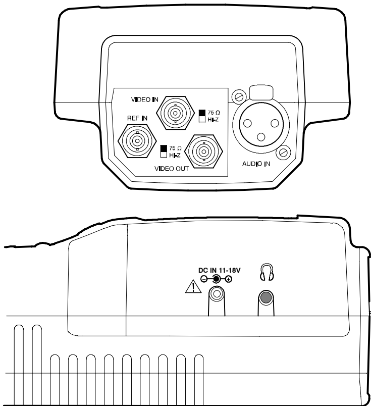
Figure 2-2: WFM90D and WFM91D side panels
