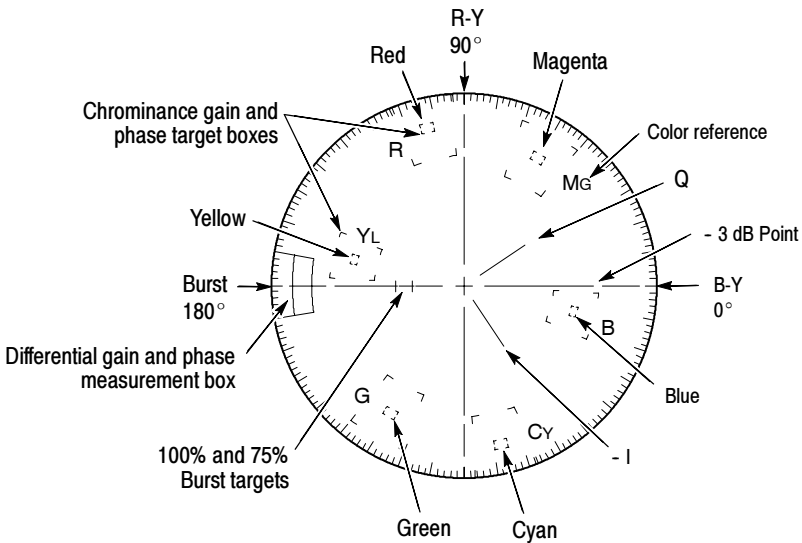
Figure 3-3: NTSC vector graticule
