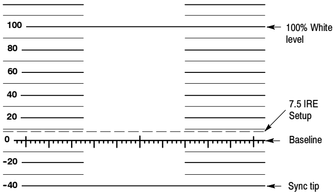
Figure 3- 1: NTSC waveform graticule
