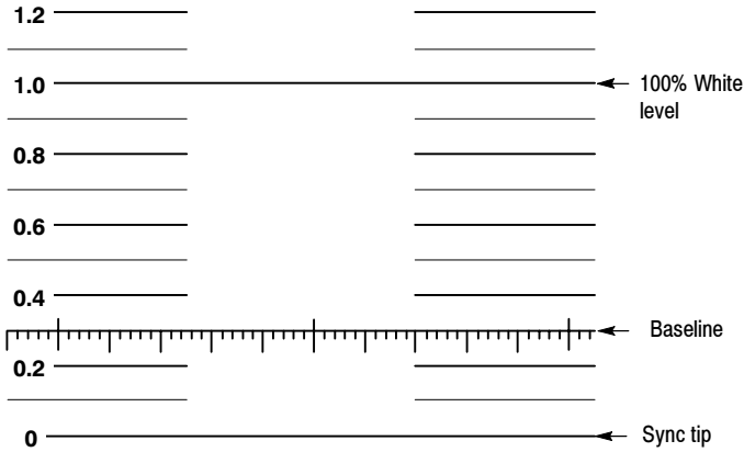
Figure 3-2: PAL waveform graticule
