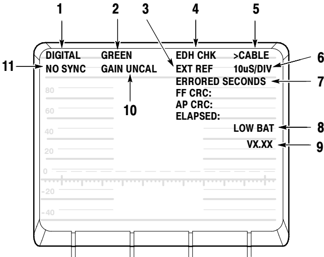
Figure 2-3: Onscreen readout messages
