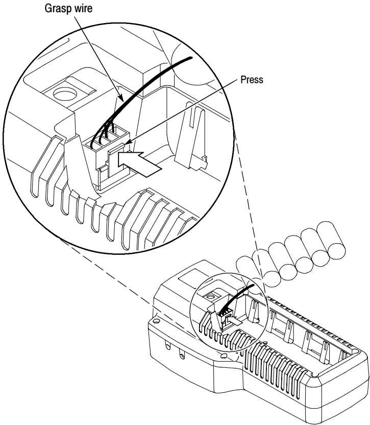
Figure 1-1: Removing the NiMH battery pack
