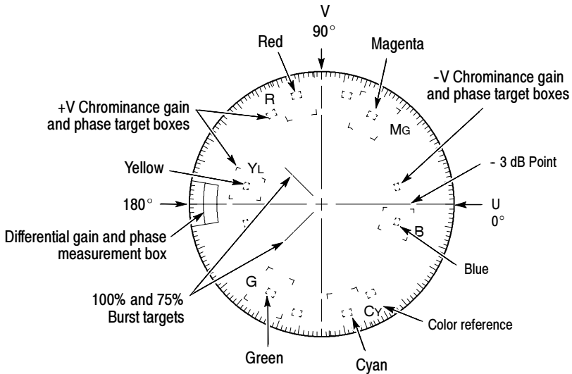
Figure 3-4: PAL vector graticule
